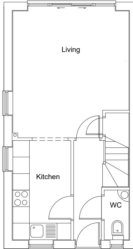
Ground Floor Plan Floor Area = 768 Ft Sq
